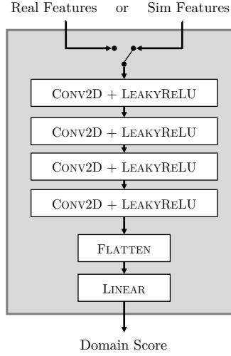
Figure 12: Our discriminator architecture. The discriminator takes as input a 3D feature map with two spatial dimensions and one feature dimension. It processes the feature map with a cascade of four convolutional neural networks with LeakyReLU non-linearities, before processing the output with a linear neural network layer. The discriminator is trained to output a scalar score that assigns high values to feature maps from the simulated domain, and low values from the real domain. The discriminator is used as component in our Wasserstein domain loss \mathcal{L}_W .
