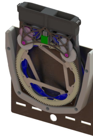
Fig. 7. The Torq gripper in its docking station. Due magnetic and gravitational force, the tool settles into a unique position.
